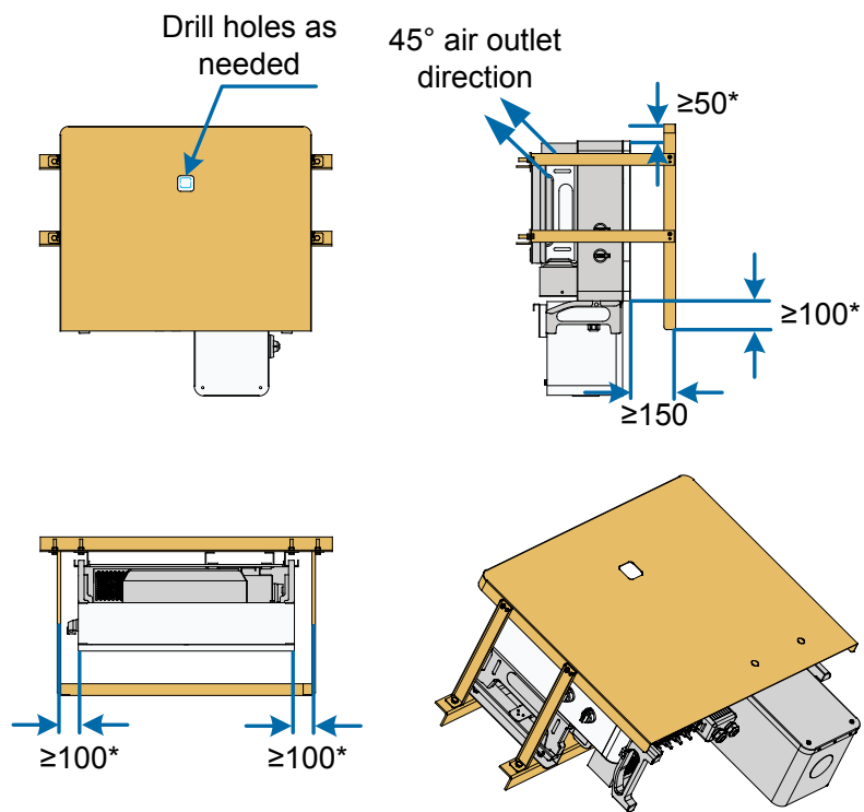
Fig. 6-7 SG36/60CX-US sunshade dimension drawing (unit: mm)
