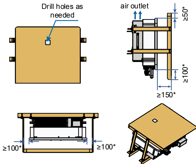
Fig. 6-9 SG25/30/33/36/40/50CX-P2 sunshade dimension drawing (unit: mm)
