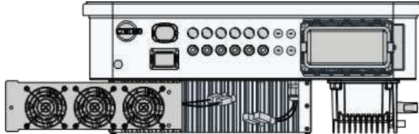
Fig. 7-10 SG15/20/25CX-P2-LV fan dimension drawing (unit: mm)
