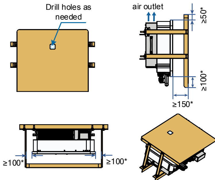
Fig. 6-10 SG15/20/25CX-P2-LV sunshade dimension drawing (unit: mm)
