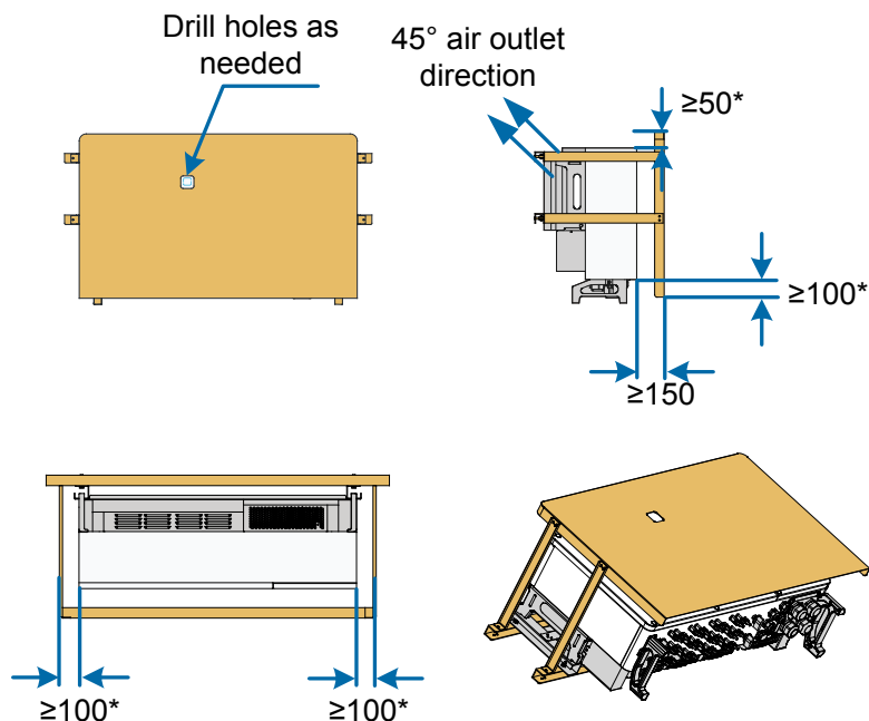
Fig. 6-8 SG100CX/SG110CX/SG136TX sunshade dimension drawing (unit: mm)
