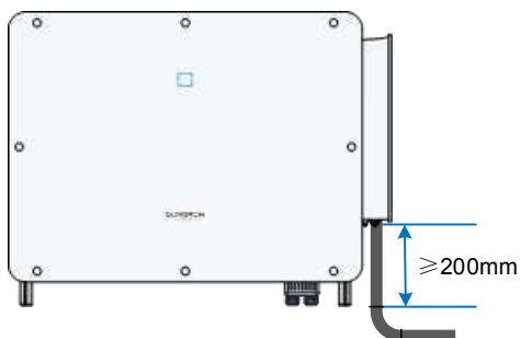
Fig. 3-16 SG75/110/125CX-P2
