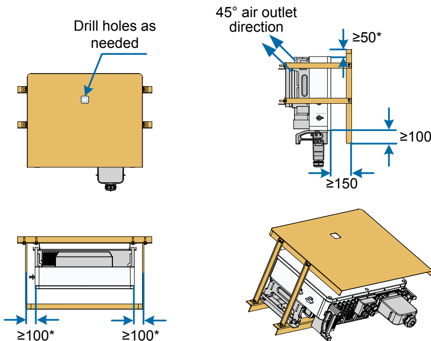
Fig. 6-6 SG25CX-SA/SG30CX/SG33CX/SG40CX/SG50CX sunshade dimension drawing (unit: mm)
